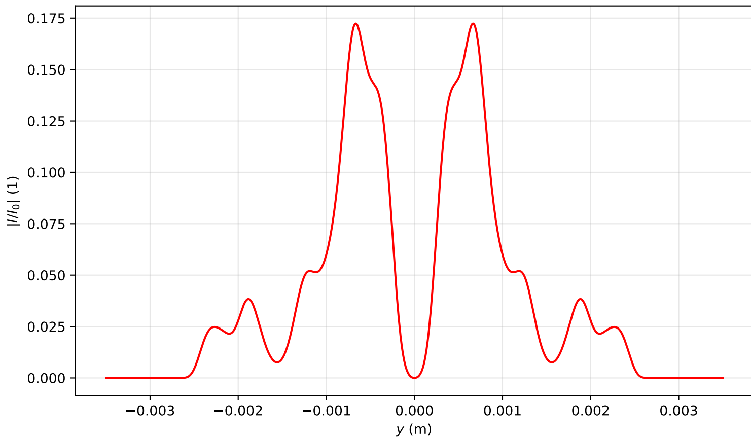
Intensity profile I(x=0, y, z=3.423)/I_0 , \text{Pin}=9.0\text{Pcr} , artificial time
